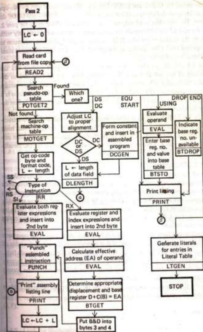
FIGURE 3.11 Detailed pass 2 flowchart
